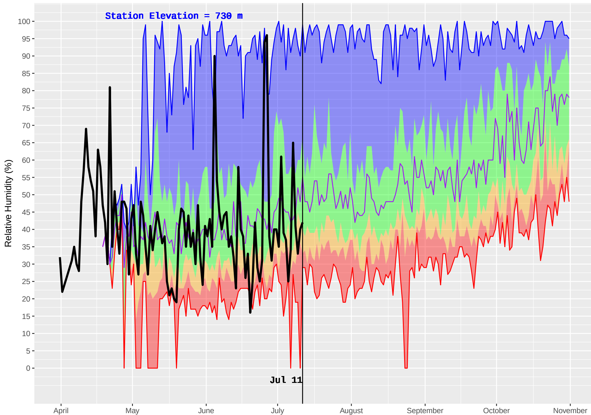
BOYA LAKE (445) : Historical (1985–2016) and Current (2018) Noon Relative Humidity
